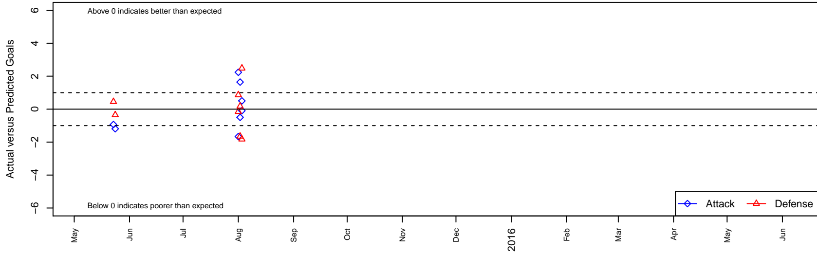
FC Golden State 05 PDA B04 Dots are actual minus expected GF (blue circles) and GA (red triangles). Blue line is smoothed change in attack strength. Red is smoothed change in defense strength.
